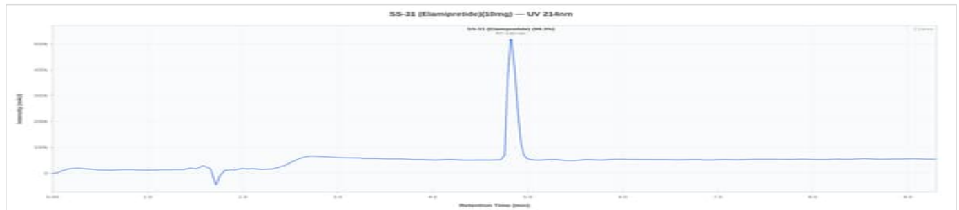
SS-31 10mg - SS99001-X: UV Chromatogram
